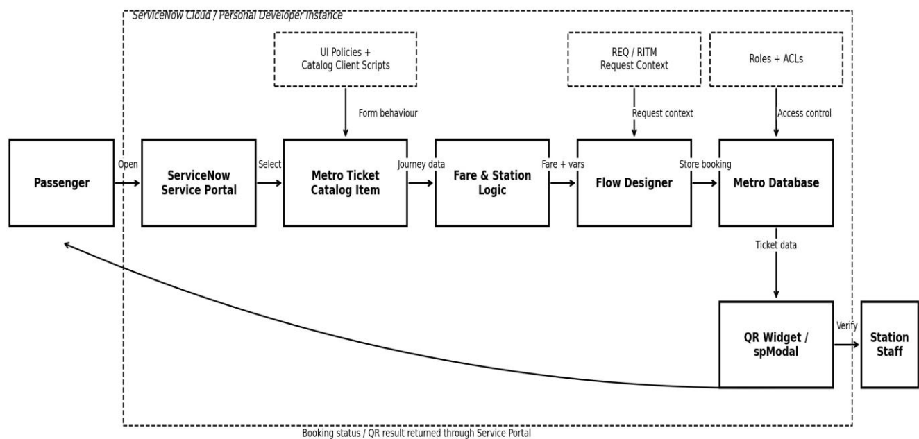
Metro Ticket Generating System - Technical Architecture
